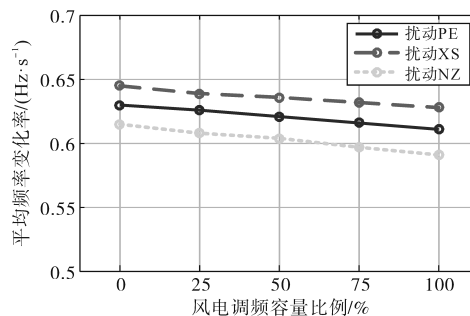
图 13 不同风电调频容量比例下的系统平均频率变化率 Fig.13 The system average frequency change rate under different ratios of wind power frequency regulation capacity
